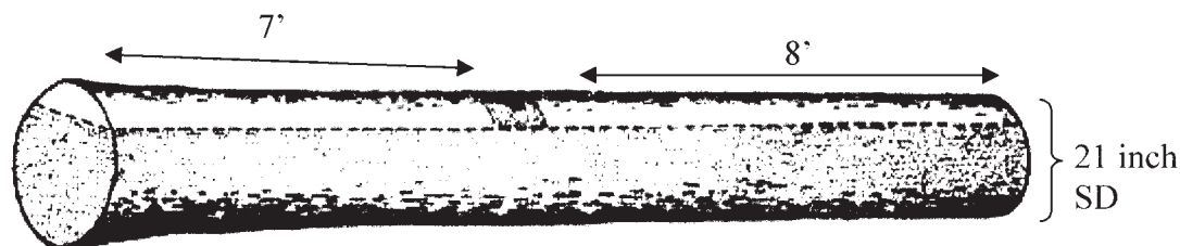
Figure 8. Example of an F1 grade, 16-foot butt-log. Adapted from Rast and others, USDA Forest Service, 1973.
