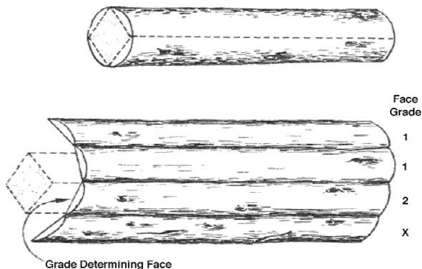
Figure 2. Establishing 4 grading faces on the butt-log. Source: Rast and others, USDA Forest Service, 1973.
