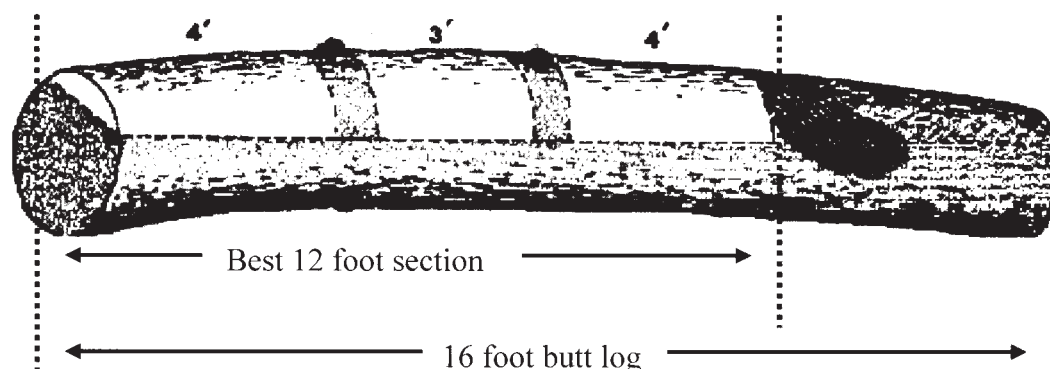
Figure 9. An example of an F2 grade butt-log. Adapted from Rast and others, USDA Forest Service, 1973.
